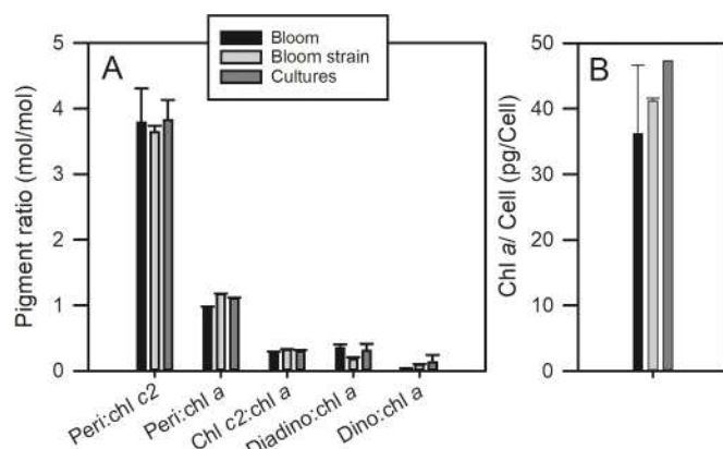
Fig. 12. Pigment composition of Lingulodinium polyedra in the bloom and in monoalgal cultures. (A) Pigment ratios (mol/mol): Peridinin/Chl c2, Peridinin/Chl a, Chl c2/Chl a, Diadinoxanthin/Chl a, Dinokxanthin/Chl a. (B) Chl a per cell (pg/cell). Each bar is the mean of 12 different samples for the bloom data, the mean of three different strains (LP4V, LP9V from Zapata et al. (2012) and VGO668) for the culture data and the mean of four cultures for the strain IFR-LI-01LC. Error bars represent standard deviations.
